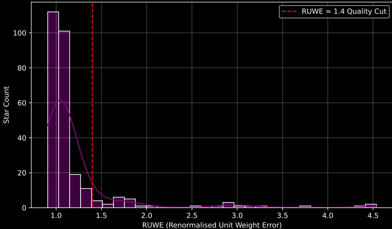
GALAH DR4 Field [6958] RUWE Distribution (n= 274)
