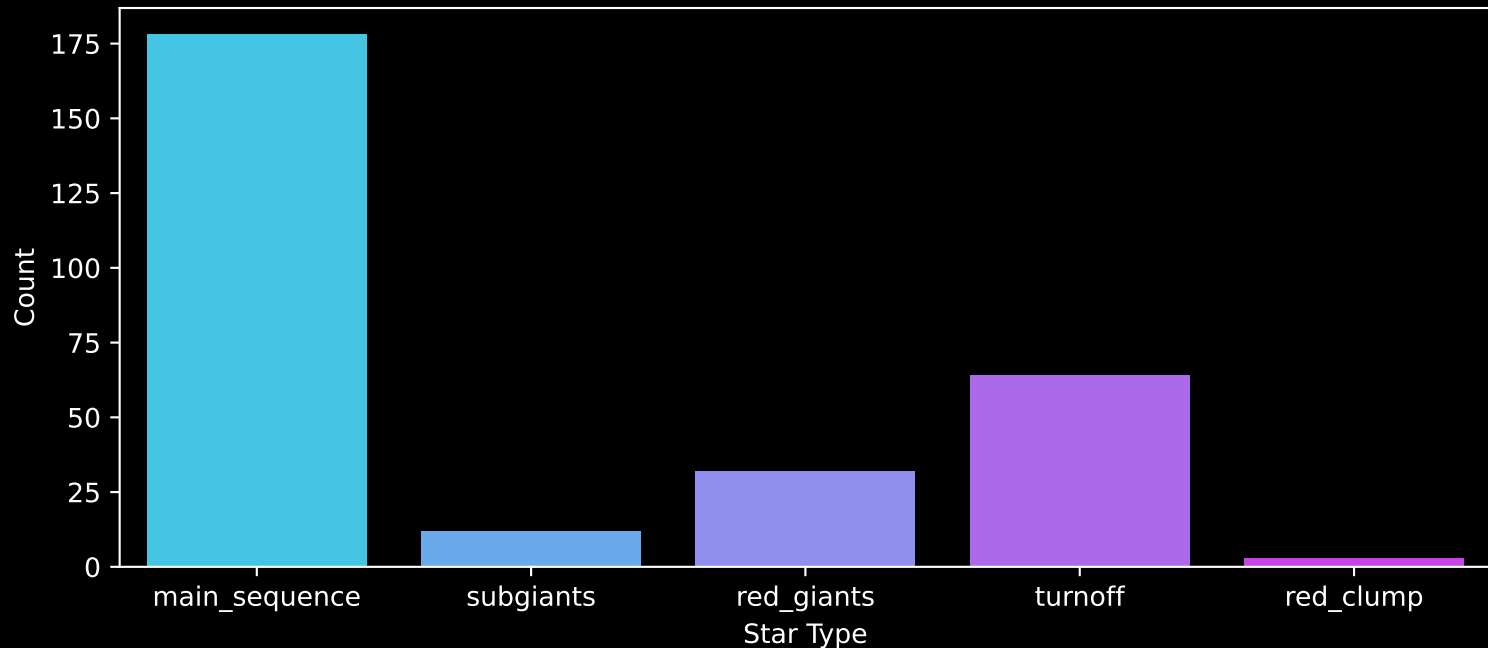
GALAH DR4 Field: [6958] Count plot of Star Type
