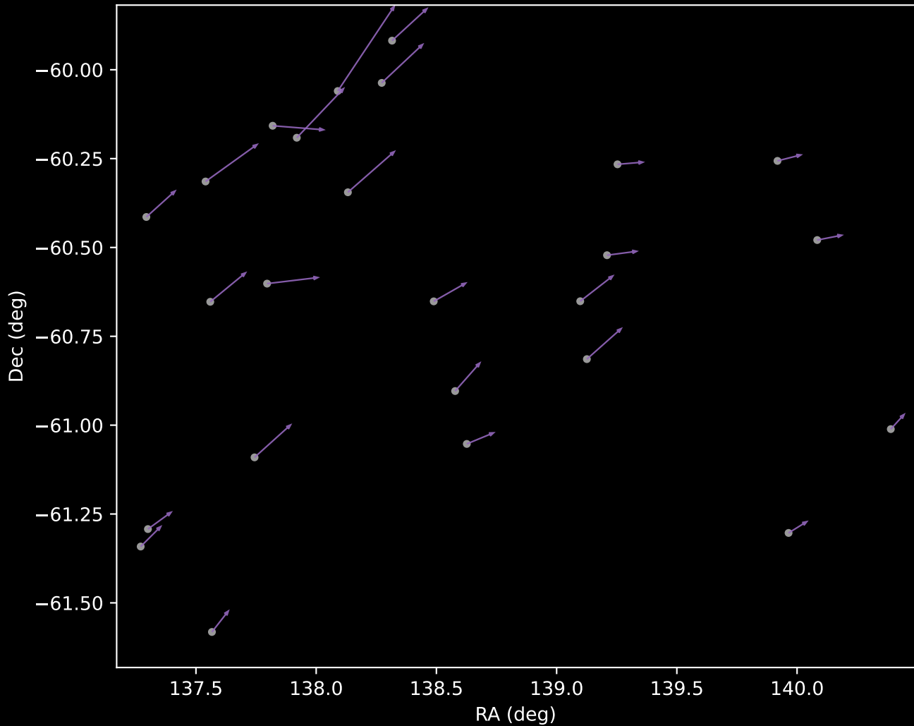
GALAH DR4 Cluster 8 Proper Motion Vectors (n=25)
