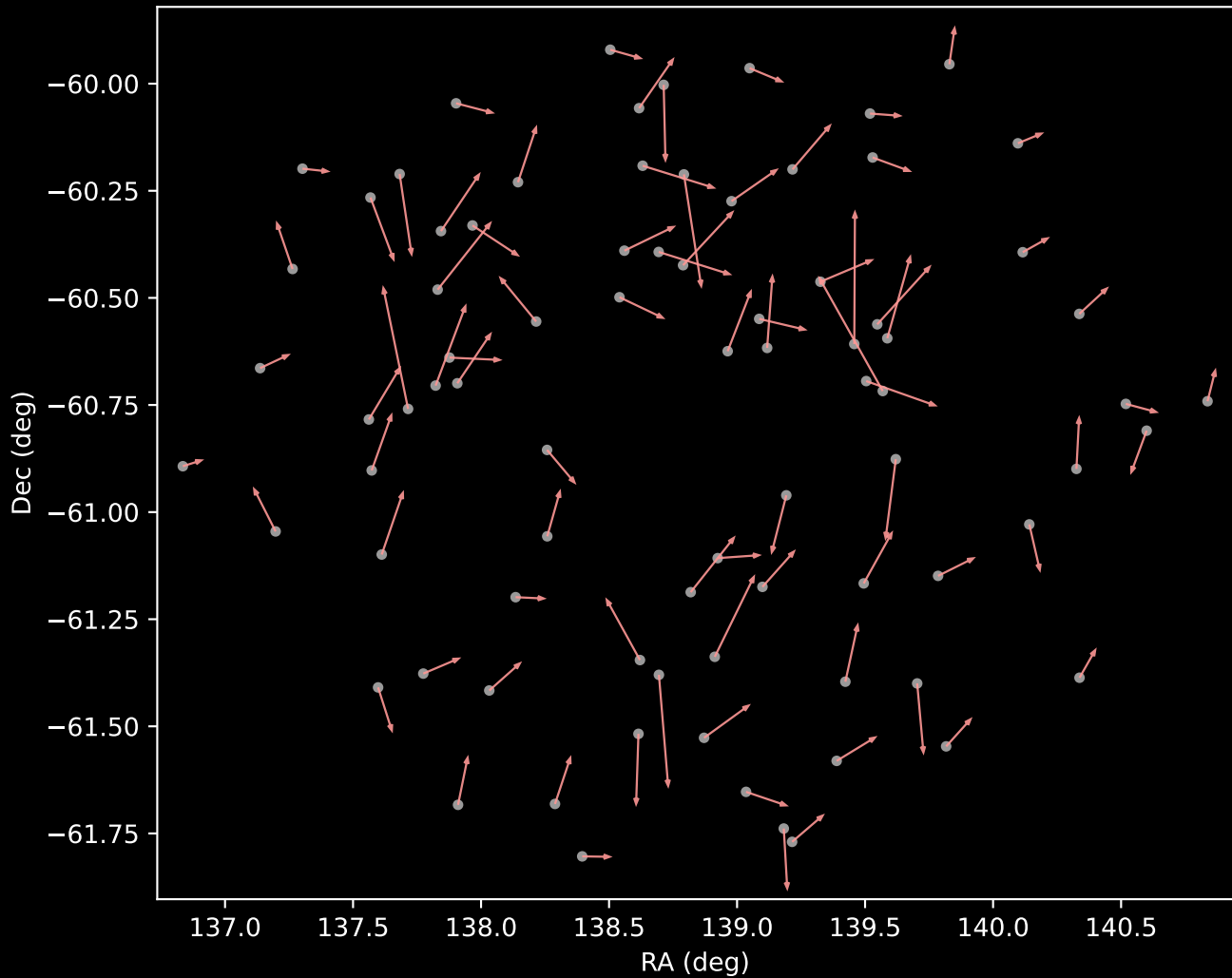
GALAH DR4 Cluster 7 Proper Motion Vectors (n=81)
